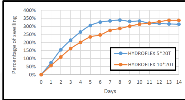
The percentage of swelling in tap water at 23 °C
